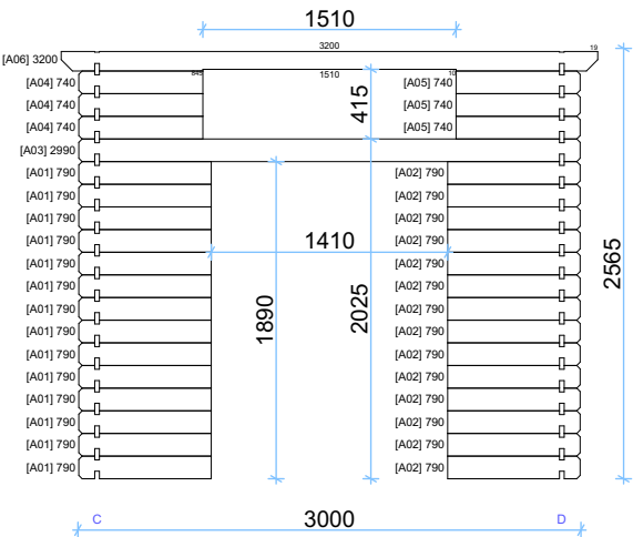
Wall A 1:50
