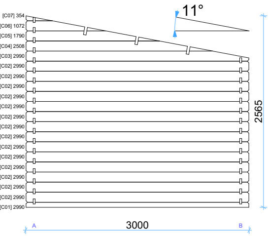
Wall C 1:50
