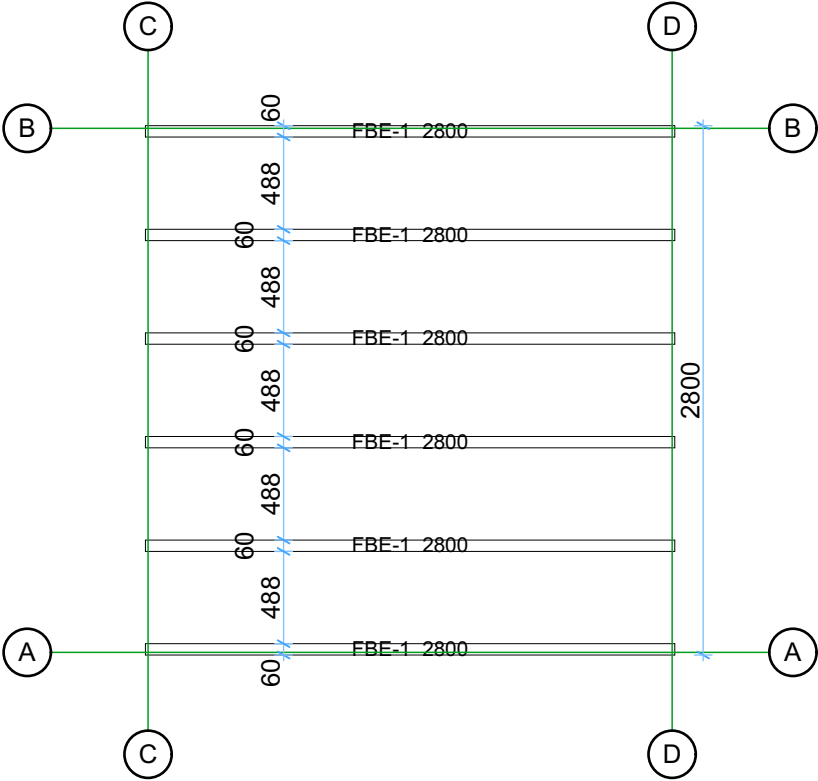
Floor bearers
